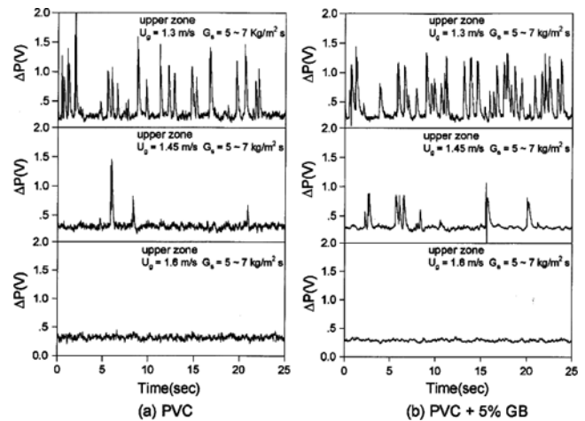
Fig. 2. Pressure fluctuation signals with different gas velocity (a) for PVC and (b) PVC+5% GB.
